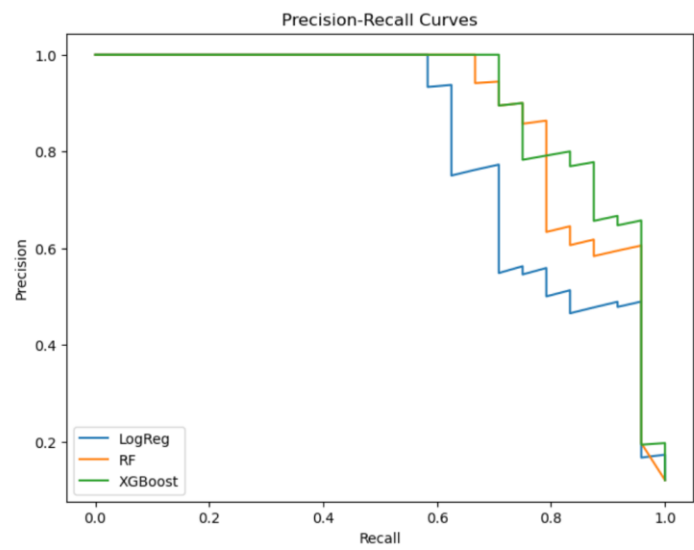
Figure 7. Precision-Recall Curves
